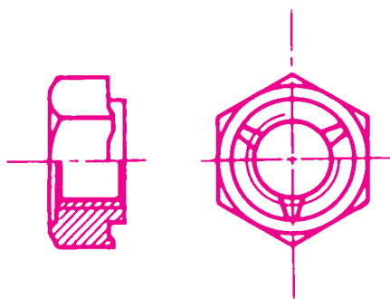
Self-locking weld nut
