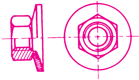
Hex nut with captive spring washer
