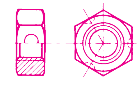
self-locking hexagon nut (din 980)
