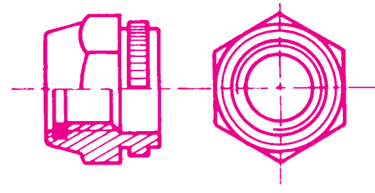
Nylon insert retreating nut
