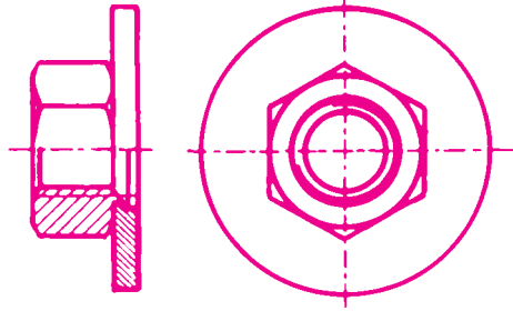
Nut with flat washer (combination)
