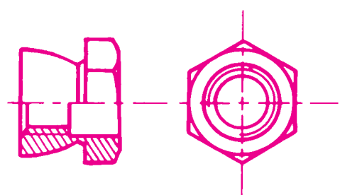
Self breaking nut
