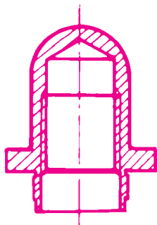
Self clinching blind nut
